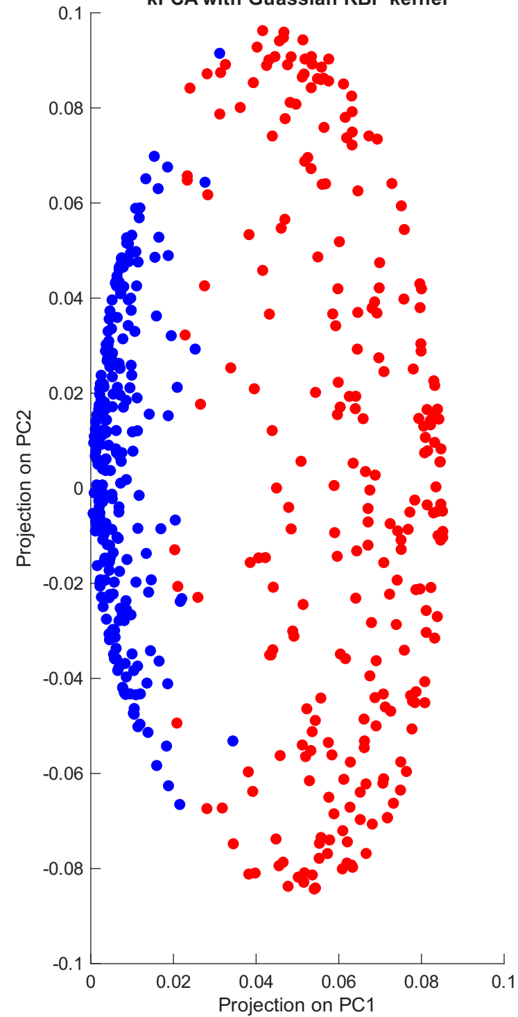
kPCA with Gaussian RBF kernel
